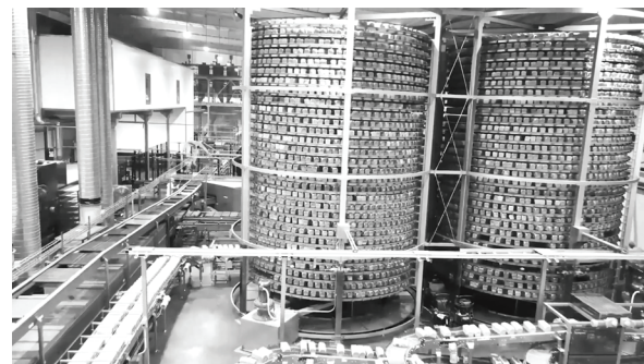
The Gardenia Cooling Tower inside the new and automated bread plant in Pampanga, the whole plant is computer-controlled starting from the use of an upgraded concept in the ingredient handling and makeup systems, proofing, use of robotics in handling baking pans and a unique technology in the depanning process which promises to be gentle to the bread, completely untouched by human hands. (Photo Courtesy of Media Blitz)
